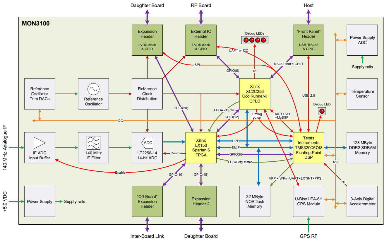
MON3100 Compact Low Power Wireless Baseband Processor Block Diagram
